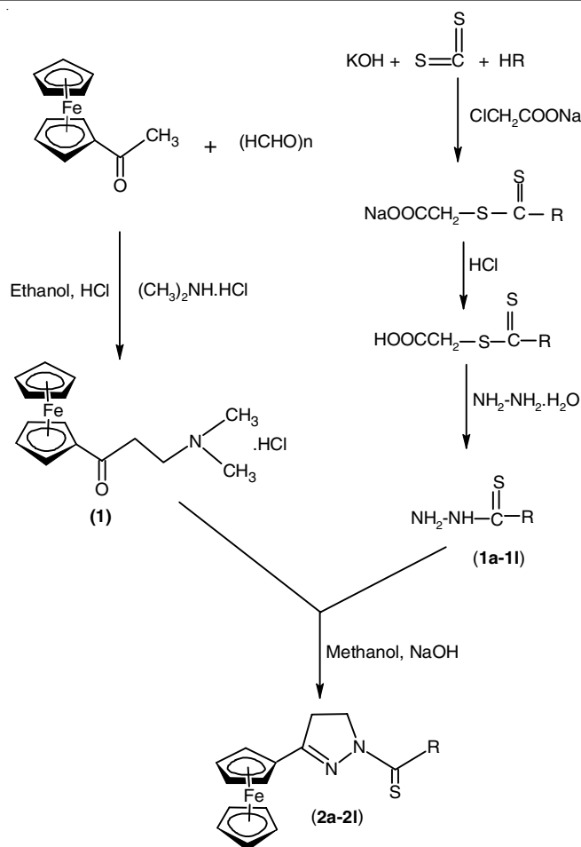
Scheme-I: General synthesis of 1- N -substituted thiocarbamoyl-3-ferrocenyl-2-pyrazoline derivatives (2a-2l)
