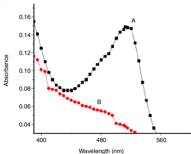
Fig. 2. Absorption spectrum of Fe(II)-DMG-pyridine complex (Conditions: Fe(III) = 100 \mu g, vitamin E = 50 \mu g, DMG solution = 2.0 mL, pyridine = 2.0 mL), A = Measured against blank, B = Blank measured against water
