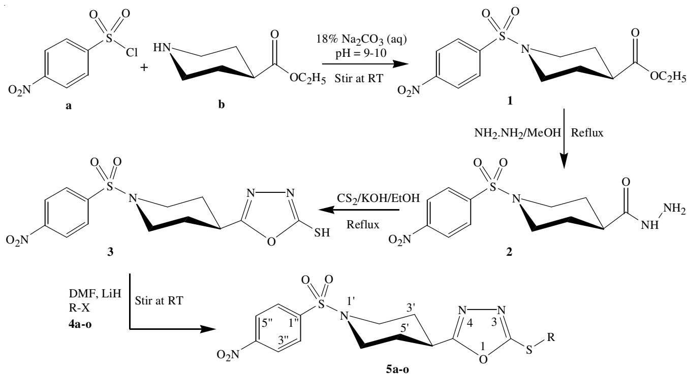
Scheme-I: Synthesis of 2-(substituted thio)-5-[1-(4-nitrophenylsulfonyl)piperidin-4-yl]-1,3,4-oxadiazole ( 5a-o )
