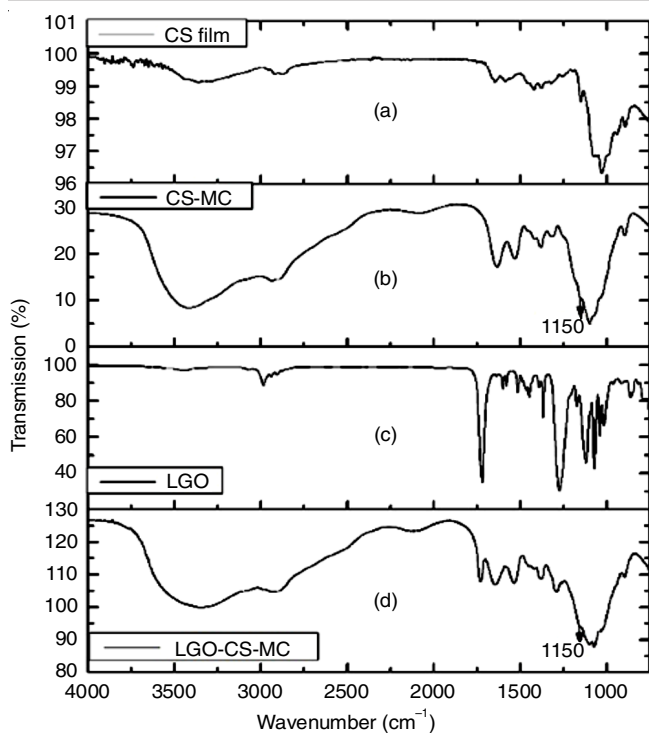
Fig. 5. FTIR spectra of LGO, CS film, CS-MC and LGO-CS-MC
