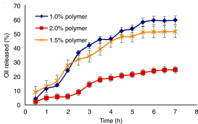
Fig. 7. Effect of variation of CS concentration on release profile
