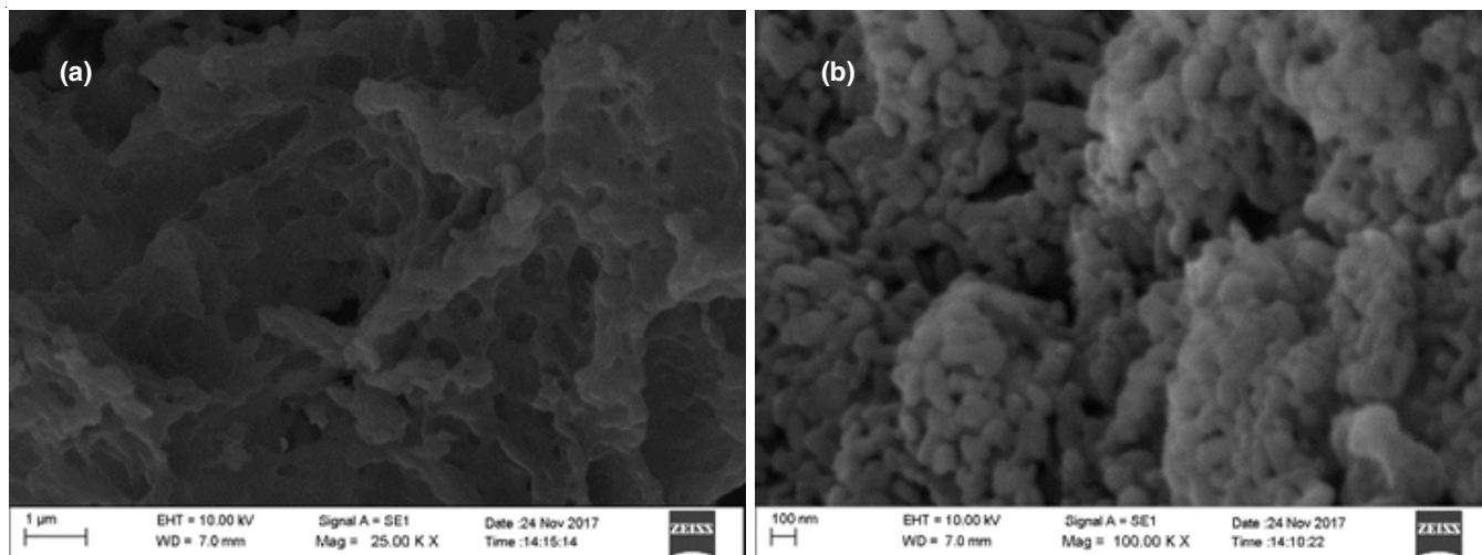
Fig. 4. Scanning electron microscopic images of (a) CS-MC (1.0 g of CS, 0.5 g of STPP) (b) LGO-CS-MC (3.0 g of LGO, 1.0 g of CS, 0.5 g of STPP)
