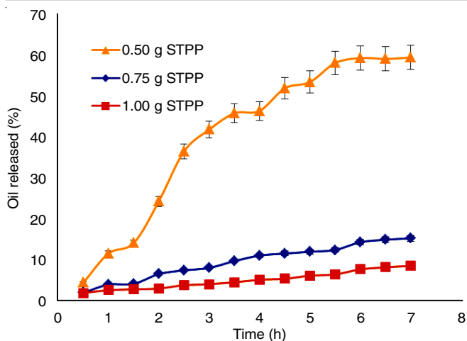
Fig. 8. Effect of variation of STPP concentration on release rate
