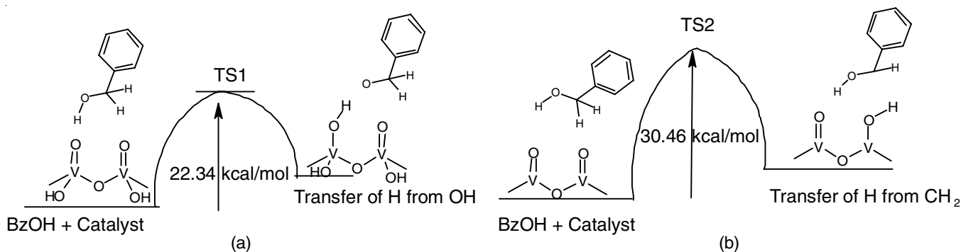
Fig. 7. Schematic PES diagram for hydrogen abstraction by the catalyst from (a) OH group (b) \text{CH}_2 group of benzyl alcohol
