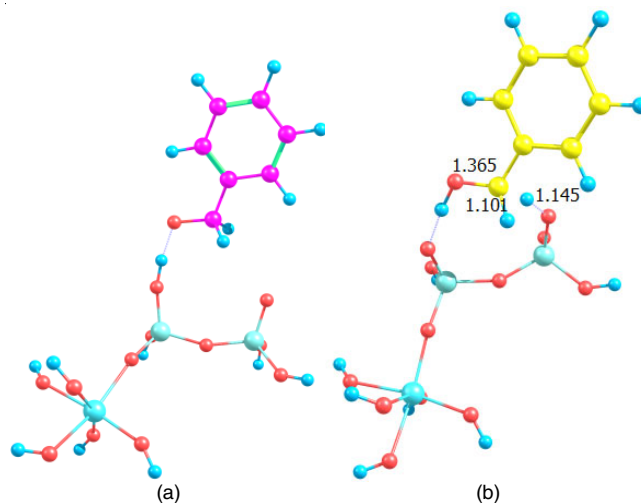
Fig. 8. Hydrogen abstraction by the catalyst from (a) OH and (b) \text{CH}_2 groups of benzyl alcohol
