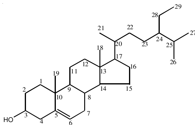
Structure of \beta -sitosterol
