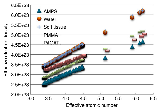
Fig. 5. Relation between Effective atomic number and electron density
