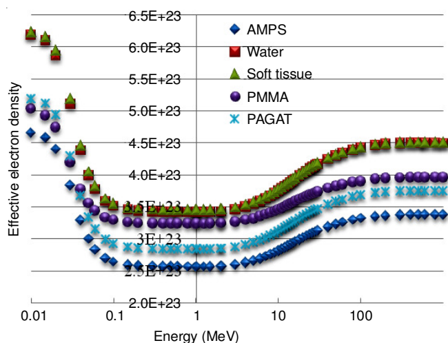
Fig. 3. Energy dependent effective electron density for PAGAT, AMPS, PMMA, soft tissue and water
