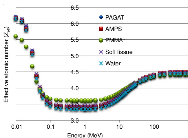
Fig. 1. Energy dependent effective atomic number for PAGAT, AMPS, PMMA, soft tissue and water
