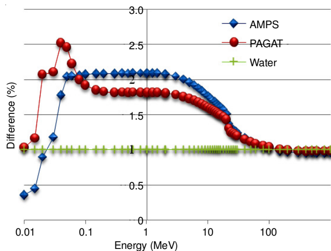
Fig. 6. Variation in the effective atomic number of AMPS and PAGAT with respect to water
