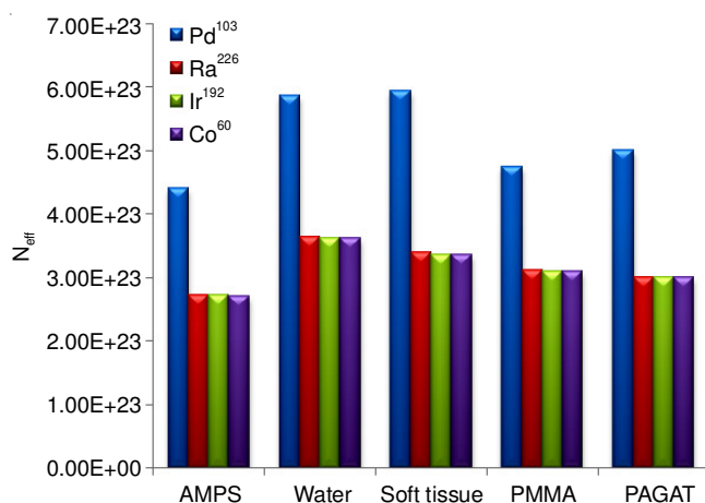
Fig. 4. Energy dependent effective electron density of PAGAT, AMPS, PMMA, soft tissue and water for \text{Pd}^{103} , \text{Ra}^{226} , \text{Ir}^{192} and \text{Co}^{60}
