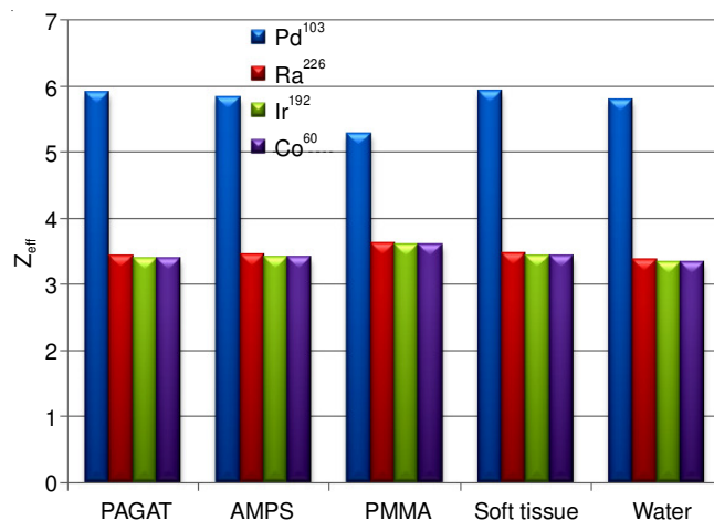
Fig. 2. Energy dependent effective atomic number of PAGAT, AMPS, PMMA, soft tissue and water for Pd 103 , Ra 226 , Ir 192 and Co 60
