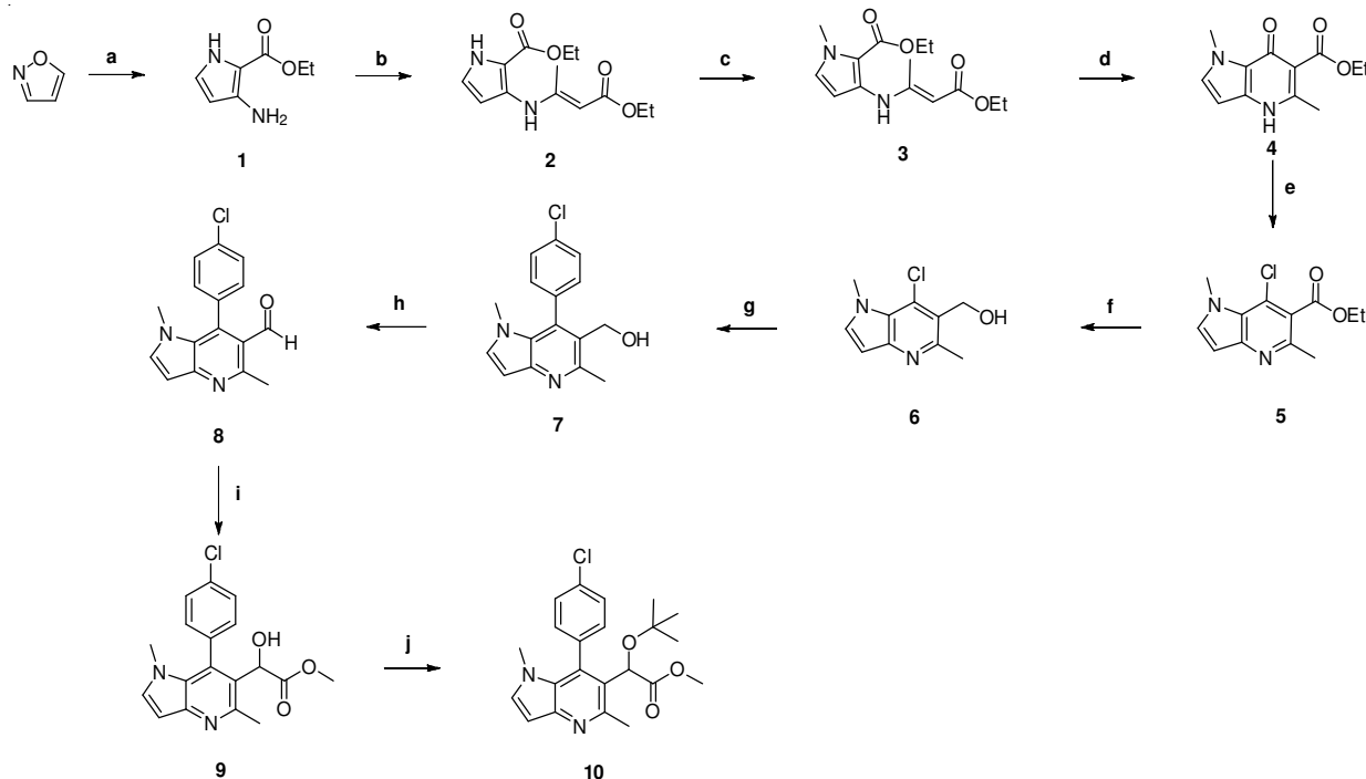
Scheme-II: Synthesis of pyrrolo-pyridine derivatives 11a-c
