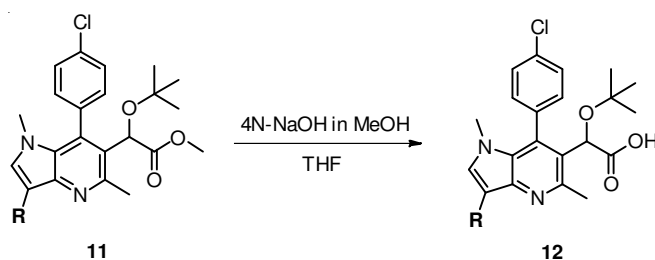
Scheme-IV: Synthesis of final products 12a-j
