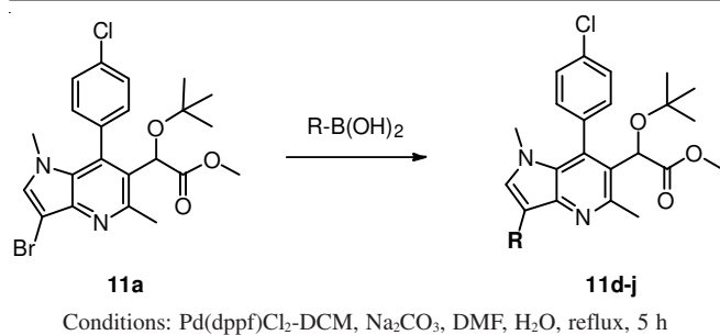
Scheme-III: Synthesis of pyrrolo-pyridine derivatives 11d-j
