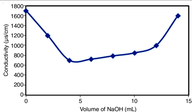
Fig. 2. Conductometric titration curve of deacetylated chitosan
