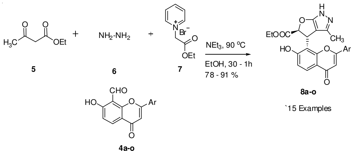
Scheme-II: Synthesis of dihydro-1 H -furo[2,3- c ]pyrazole flavones
