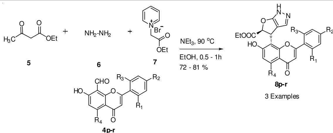
Scheme-III: SAR oriented synthesis of furo[2,3- c ]pyrazole-flavone hybrids ( 8p-r )
