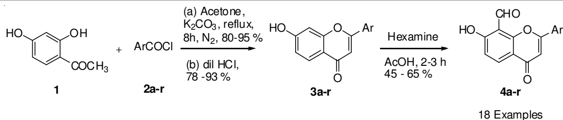
Scheme-I: Formylation of 7-hydroxy, 8-formyl flavones
