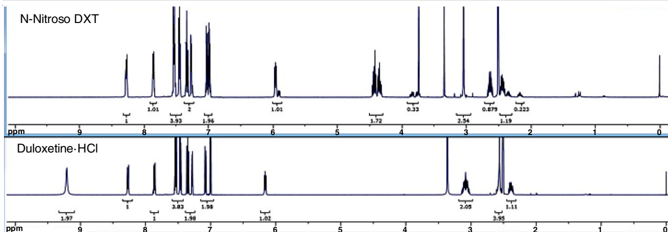
Fig. 3. Overlay of ^1\text{H} NMR spectrum of duloxetine. HCl and N-nitroso duloxetine
