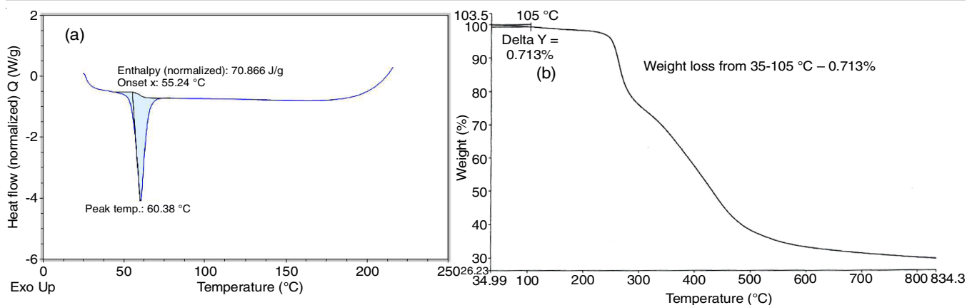
Fig. 13. (a) DSC and (b) TGA thermogram of N-nitroso duloxetine
