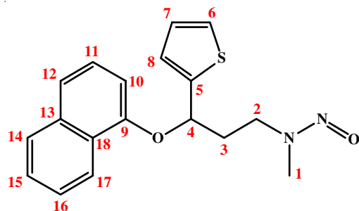
Fig. 9. Numbering assignment of N-nitroso duloxetine
