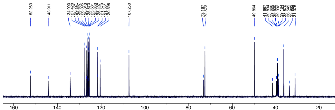
Fig. 8. ^{13}\text{C} NMR spectrum of N-nitroso duloxetine
