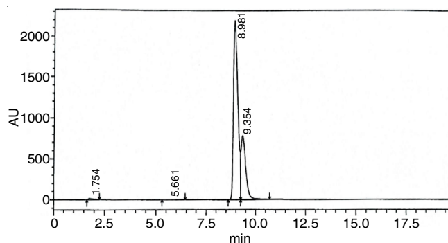
Fig. 4. HPLC chromatogram of N-nitroso duloxetine
