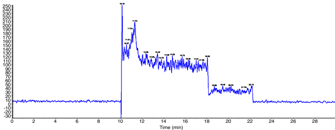
Fig. 14. Blank chromatogram of N-nitroso duloxetine
