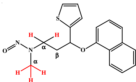
Fig. 2. Hypothetical approach on N-nitroso duloxetine
