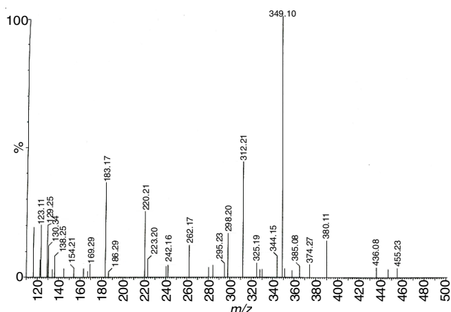
Fig. 7. Mass spectrum of N-nitroso duloxetine
