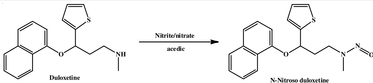
Fig. 1. Formation of N-nitroso duloxetine from duloxetine
