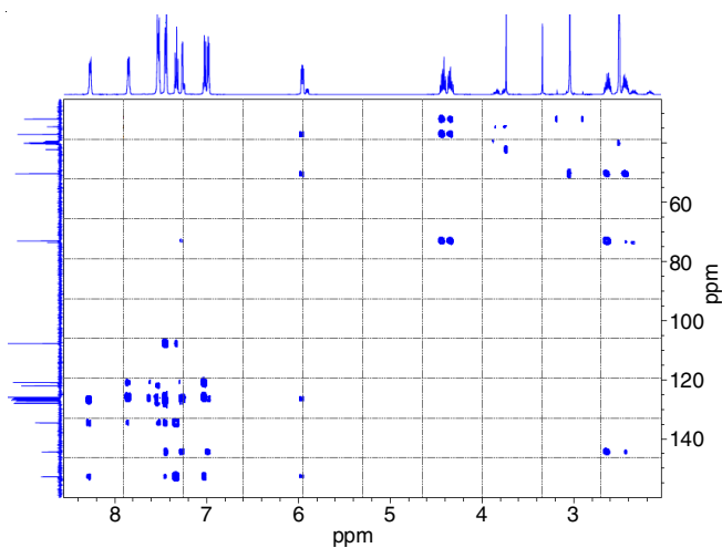
Fig. 12. HMBC spectrum of N-nitroso duloxetine
