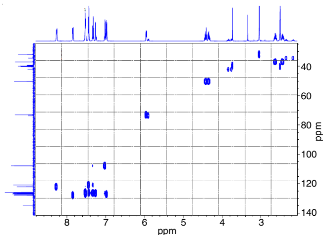
Fig. 11. HSQC spectrum of N-nitroso duloxetine
