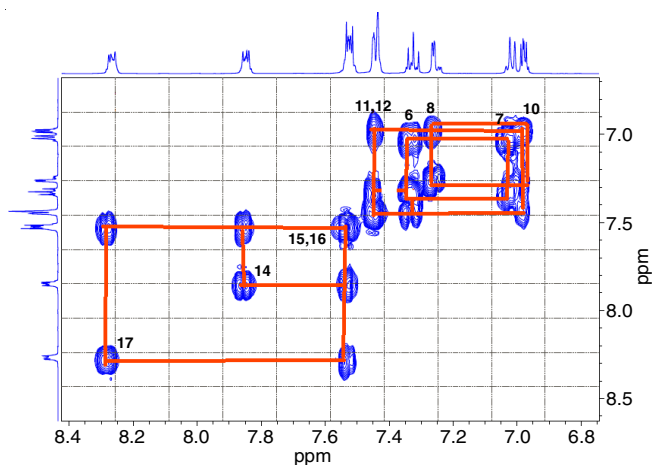
Fig. 10. COSY spectrum of N-nitroso duloxetine
