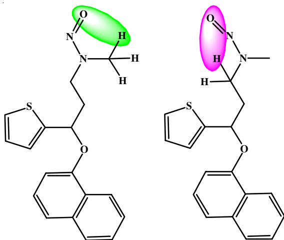
Fig. 6. Possible conformers of N-nitroso duloxetine
