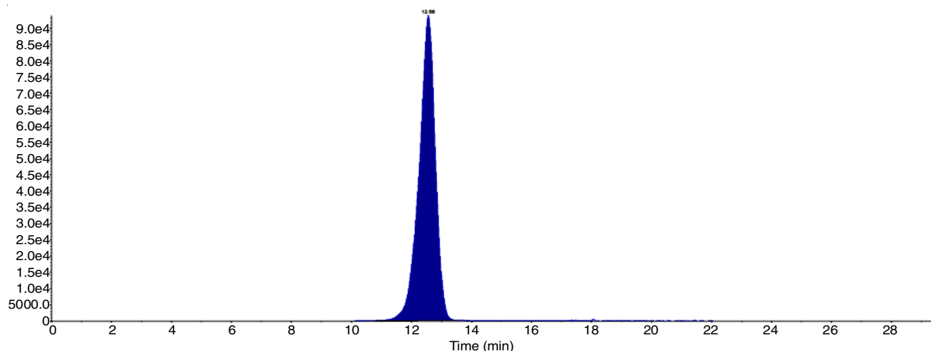
Fig. 15. Standard solution chromatogram of N-nitroso duloxetine
