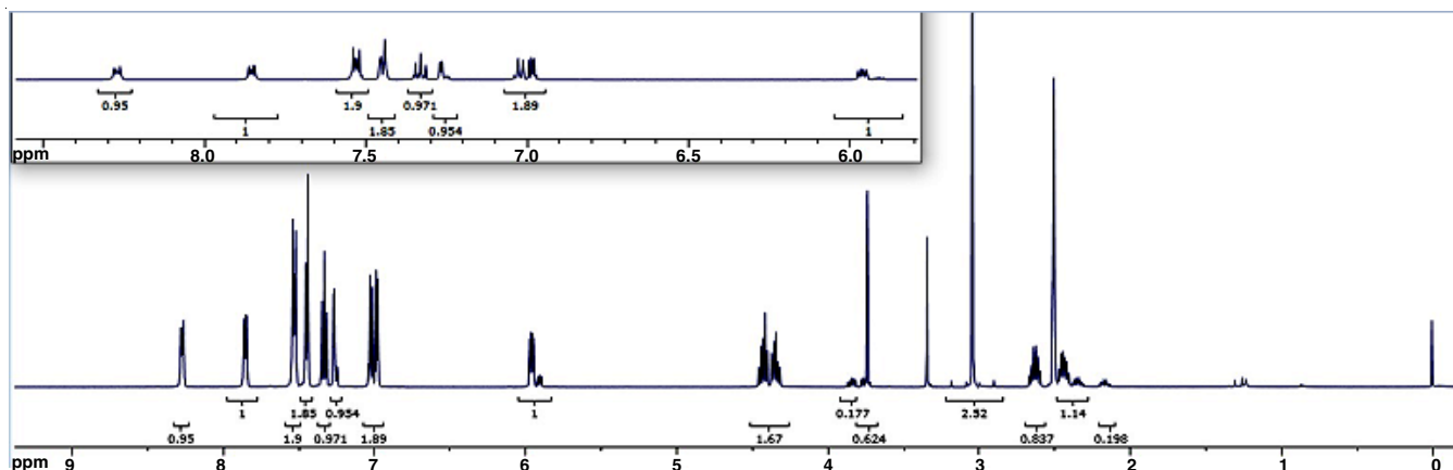
Fig. 5. ^1\text{H} NMR spectrum of N-nitroso duloxetine
