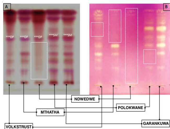
Fig. 1. Butanone eluent (a) TLC chromatogram for methanol extracts from different areas in South Africa ***DF indicates different compounds ***SM indicates same compounds. (b) Antioxidant TLC chromatogram for methanol extracts from different sites in South Africa. Rectangular dotted lines: indication of not a better resolution of compounds
