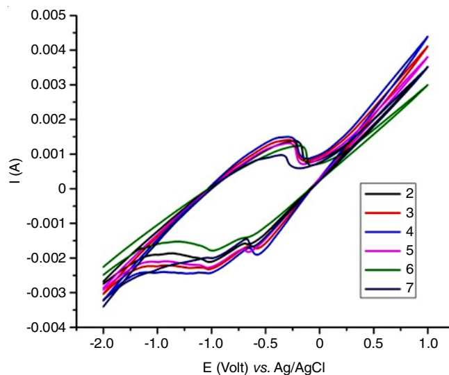
Fig. 2. Cyclic voltammogram at graphene oxide-nanozeolite composite in 0.1 M citric buffer solution (pH = 4.0) at a different pHs containing 50 ppm of aspirin and 5000 ppm potassium chloride. In all the cases, the scan rate is 100 mV s -1
