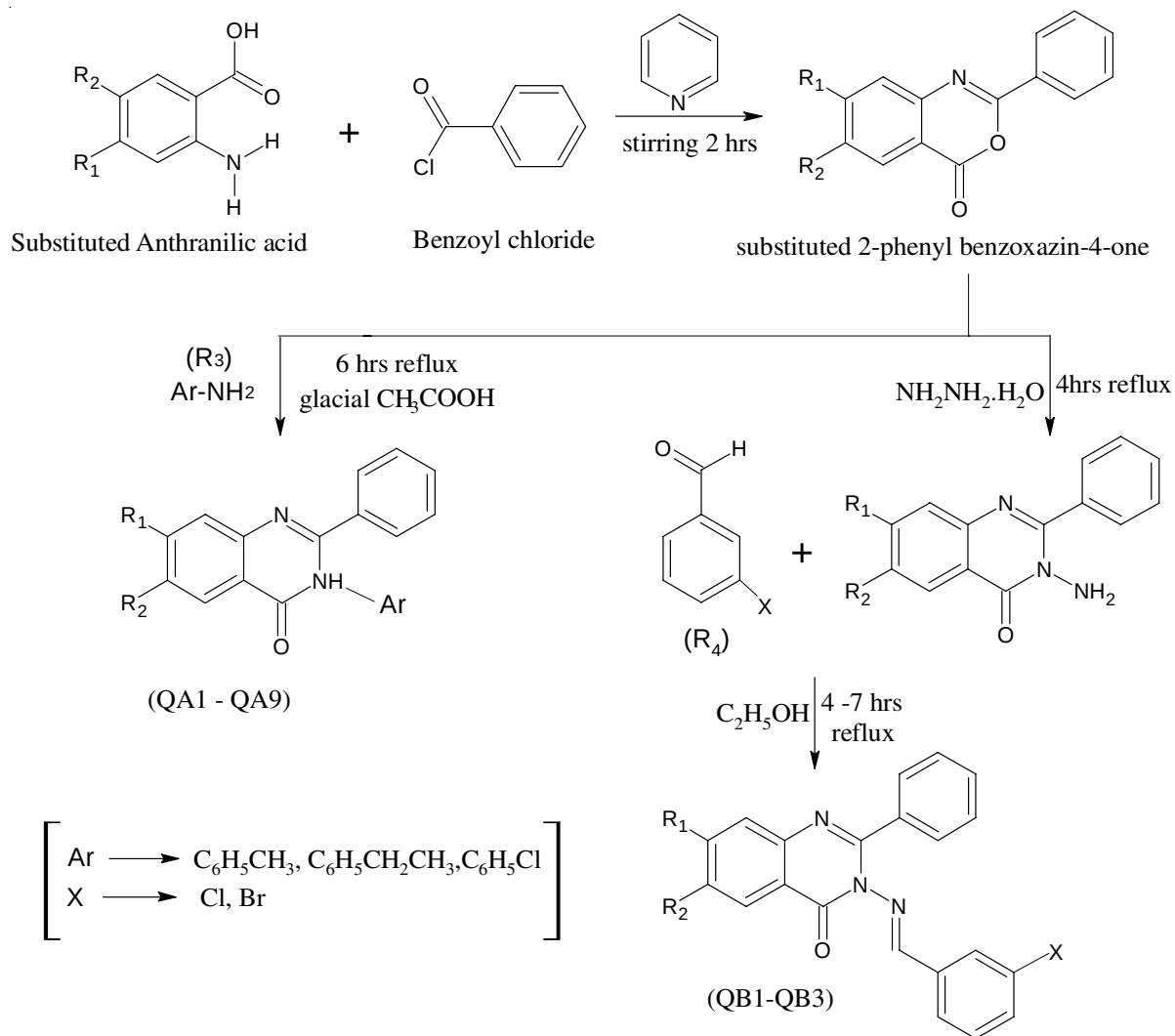
Fig. 2. Preparation of 2-phenyl-3-substituted quinazolin-4-one
