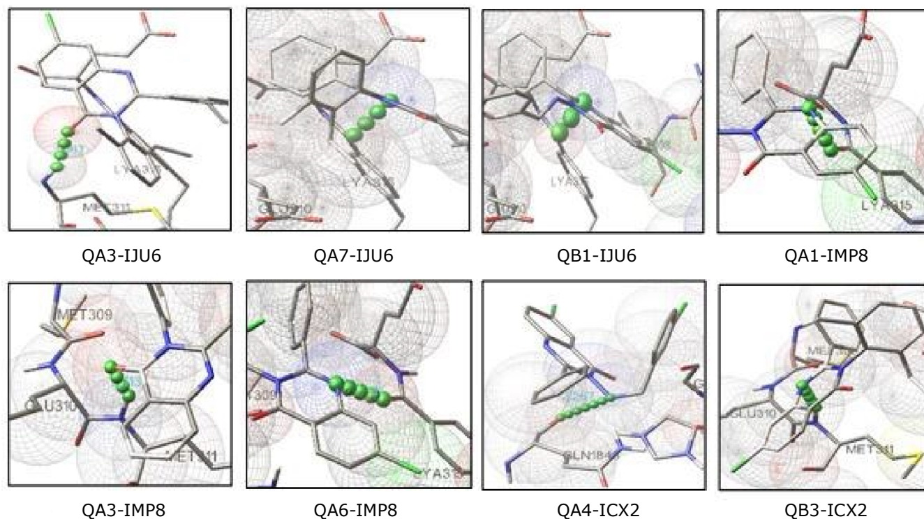
Fig. 1. Ligand-target complexes with H 2 bonding interactions by AutoDock 4.0 program
