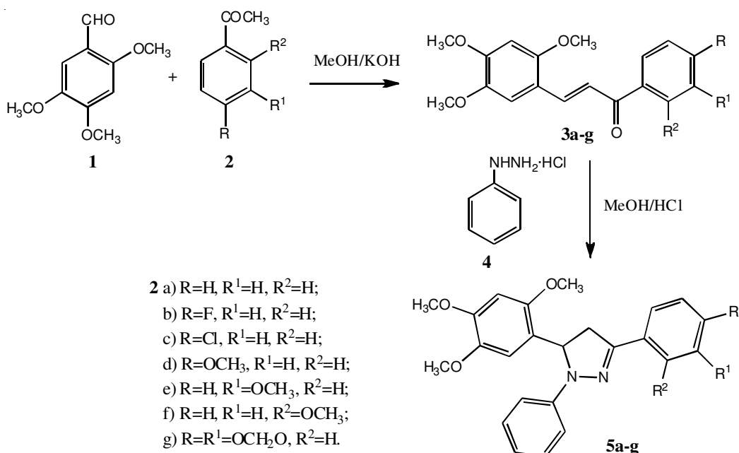
Fig. 1. Schematic diagram for the synthesis of pyrazolines ( 5a-g )
