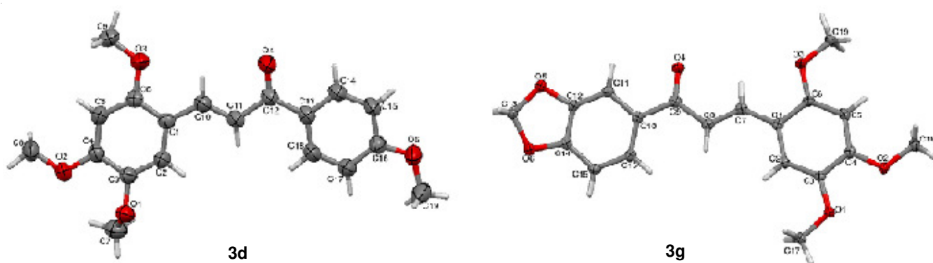
Fig. 2. ORTEP diagram of 3d and 3g with 50 % probability ellipsoids
