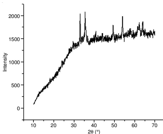
Fig. 3. XRD spectrum of ZnO nanoparticles
