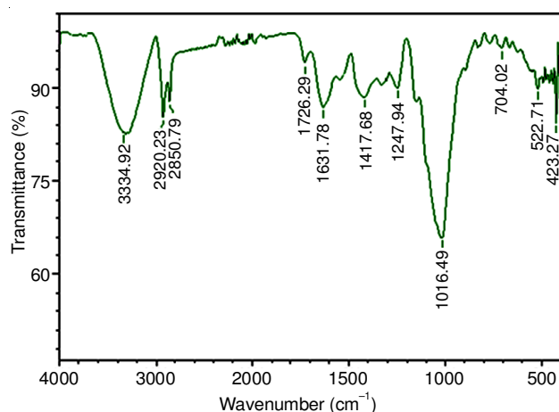
Fig. 2. FTIR spectrum of ZnO nanoparticles
