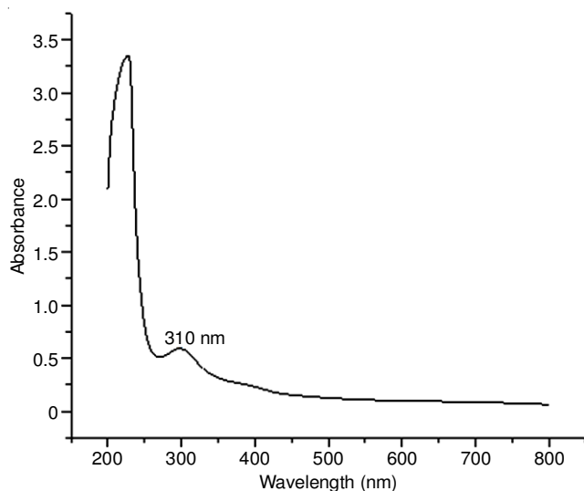
Fig. 1. UV-visible spectrum of ZnO nanoparticles
