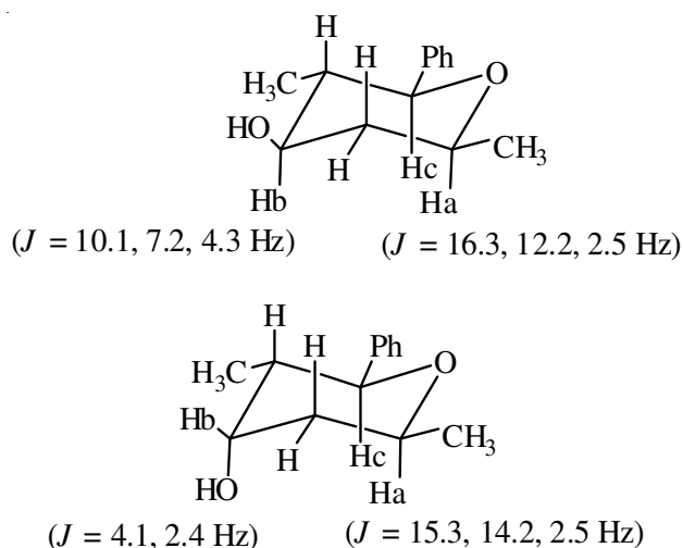
Fig. 1. Coupling constants of the products 1c and 1d
