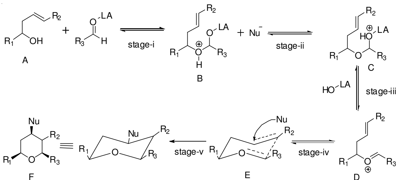
Scheme-II: General mechanisms to obtain the 1-5(c,d) cis/trans compounds from the Prins cyclization reactions
