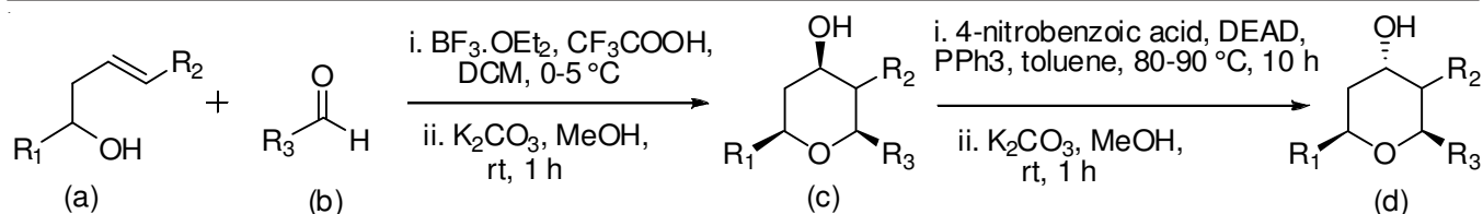
Scheme-I: Prins cyclization with \text{BF}_3\cdot\text{OEt}_2 , TFA and Mitsunobu inversion
