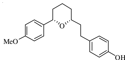
Fig. 1. (-)-Centrolobine ( 1 )
