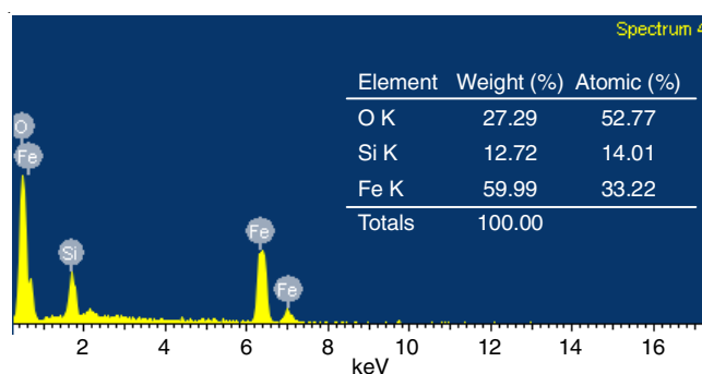
Fig 3. EDS spectra of \text{Fe}_3\text{O}_4@\text{SiO}_2
