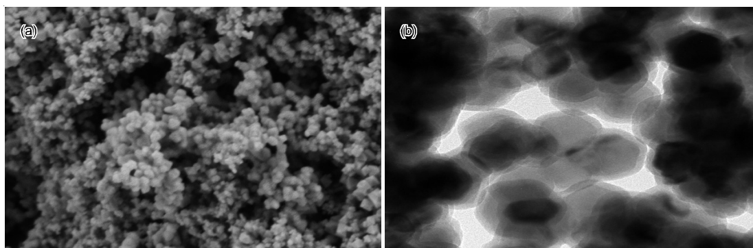
Fig 2. SEM and TEM images of \text{Fe}_3\text{O}_4@\text{SiO}_2 particles
