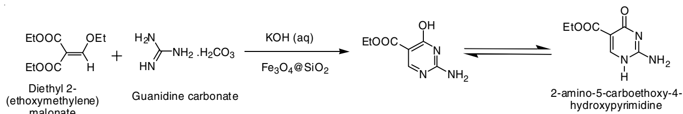
Scheme-I: Synthesis of 2-amino-5-carboethoxy-4-hydroxypyrimidine
