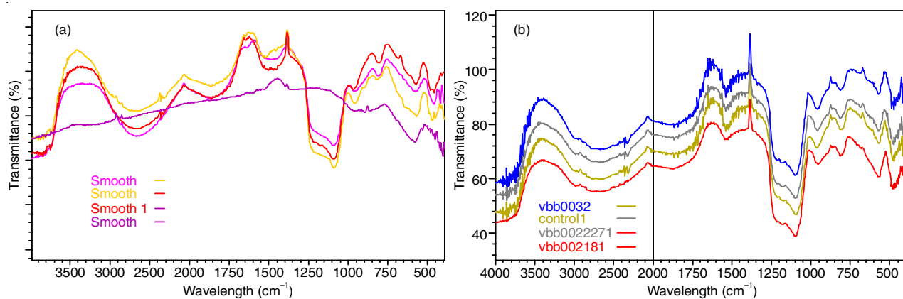
Fig 1. IR spectra of functionalized magnetic nanoparticles
