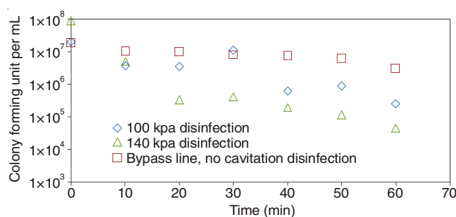
Fig. 6. Reduction in the cfu/mL of E. coli count due to cavitation using vortex diode
