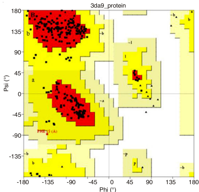
Fig. 7. Ramachandran plot
