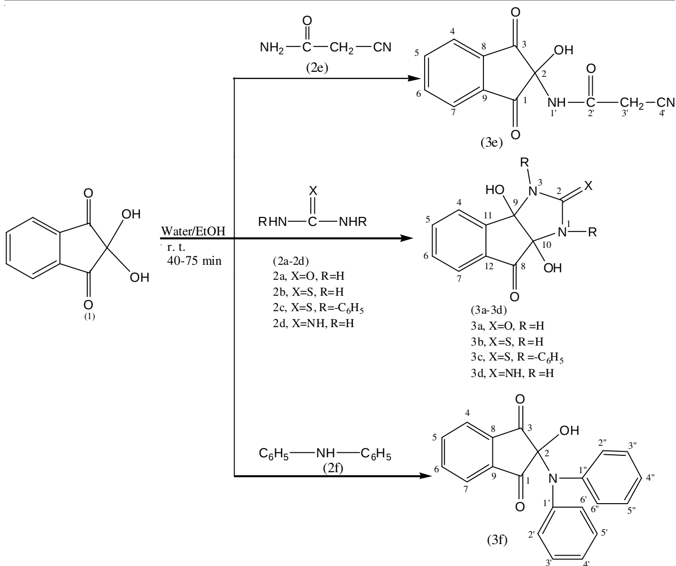
Fig. 1. Synthetic route of indeno-imidazole derivatives ( 3a-3d ) and ninhydrin-nucleophile adducts ( 3e-3f )
