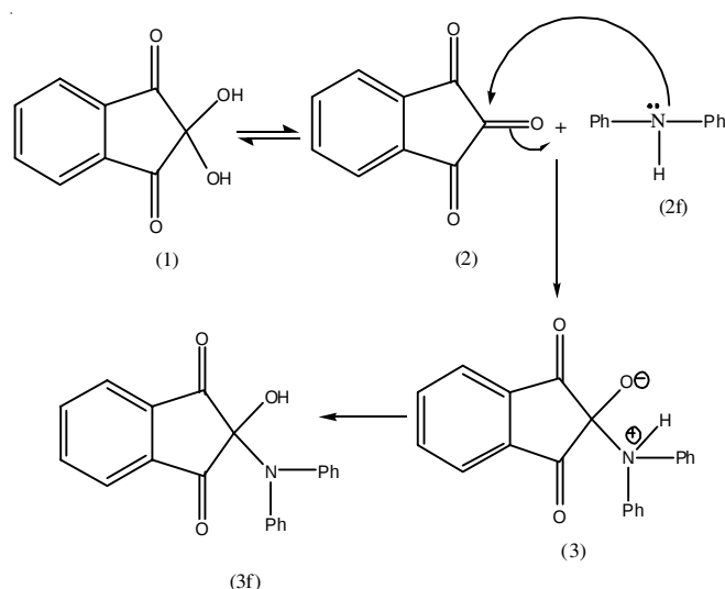
Fig. 3. Plausible reaction pathway for compounds ( 3e-3f )
