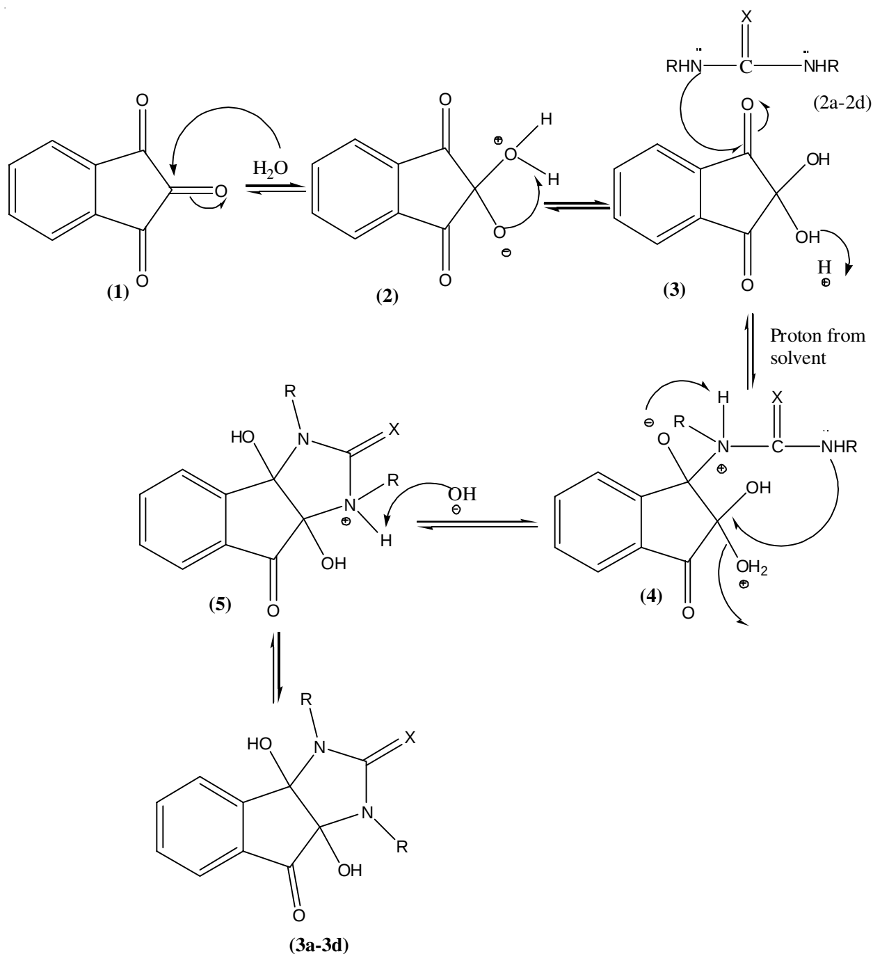
Fig 2. Plausible reaction pathway for compounds ( 3a-3d )
