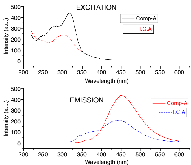
Fig. 7. Excitation and emission spectra of compound A and its inclusion complex
