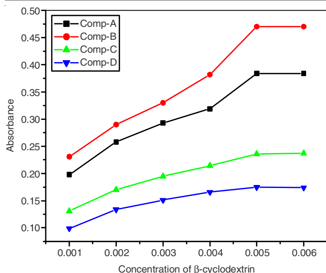
Fig. 1. Phase solubility study of the synthesized compounds in aqueous solution of \beta -cyclodextrin
