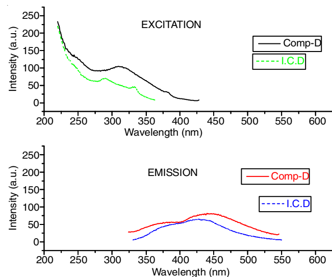
Fig. 10. Excitation and emission spectra of compound D and its inclusion complex
