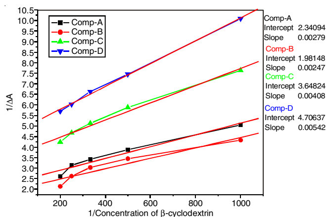
Fig. 2. Plot of inverse absorbance against inverse concentration of \beta -cyclodextrin
