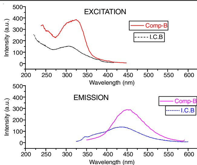
Fig. 8. Excitation and emission spectra of compound B and its inclusion complex
