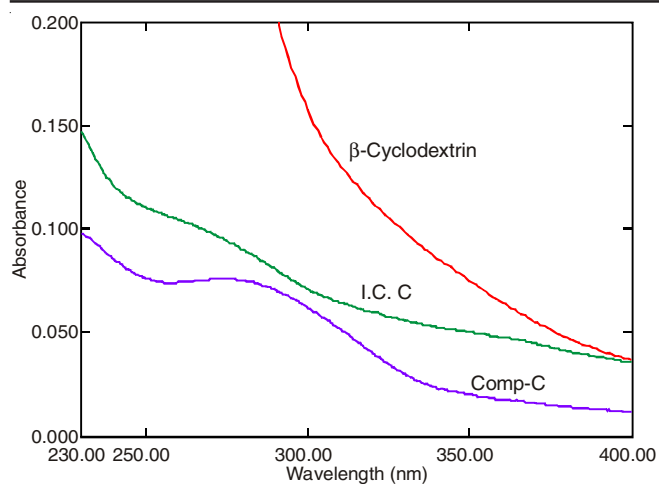
Fig. 5. UV spectrum of \beta -cyclodextrin, compound C and its inclusion complex
