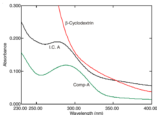
Fig. 3. UV spectrum of \beta -cyclodextrin, compound A and its inclusion complex
