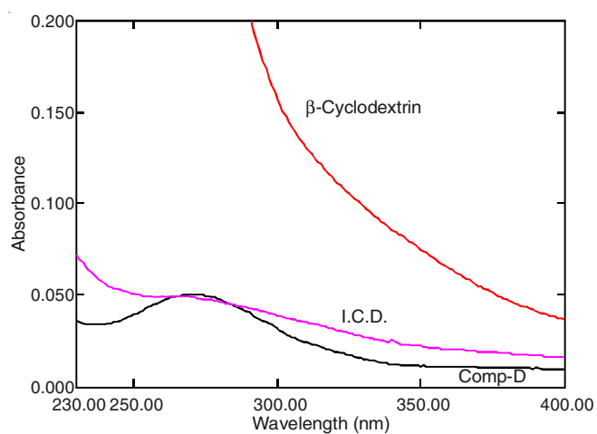
Fig. 6. UV spectrum of \beta -cyclodextrin, compound D and its inclusion complex
