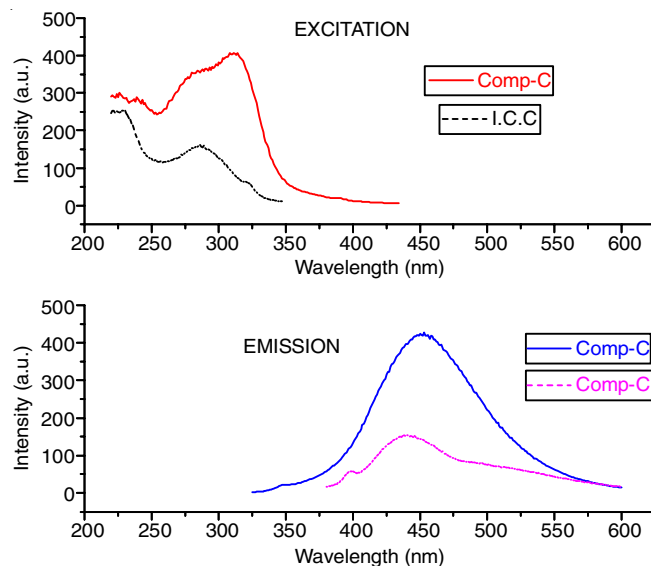
Fig. 9. Excitation and emission spectra of compound C and its inclusion complex
