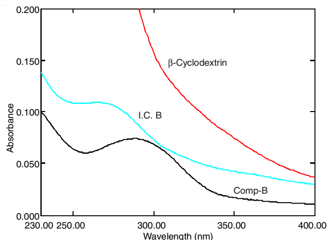
Fig. 4. UV spectrum of \beta -cyclodextrin, compound B and its inclusion complex
