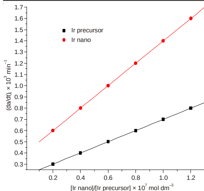
Fig. 5. Effect of [Ir nano]/[Ir precursor] on the degradation of acid red-14 by HCF(III). Experimental conditions: [acid red-14] = 3.0 \times 10^{-5} mol dm ^{-3} ; [HCF(III)] = 3.0 \times 10^{-6} mol dm ^{-3} ; pH = 7.5; Temperature = 40 \pm 0.1 °C
