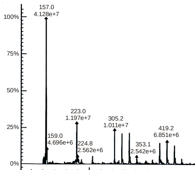
Fig. 7. LC-MS spectra of degraded products of acid red-14
