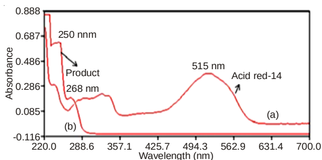
Fig. 6. UV-visible spectra of (a) acid red-14 and (b) extracted product
