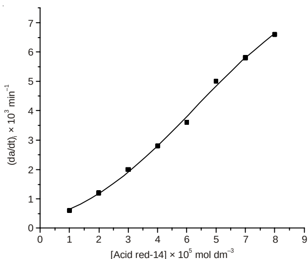
Fig. 4. Effect of [acid red-14] on the degradation of acid red-14 by HCF(III). Experimental conditions: [HCF(III)] = 3.0 \times 10^{-6} mol \text{dm}^{-3} ; [Ir nano] = 1.004 \times 10^{-7} mol \text{dm}^{-3} ; pH = 7.5; Temperature = 40 \pm 0.1 °C
