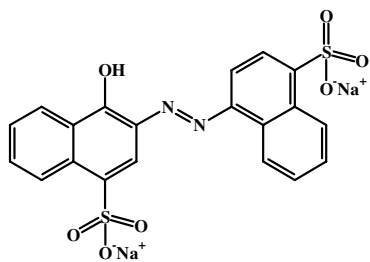
Fig. 1. Chemical structure of acid red-14
