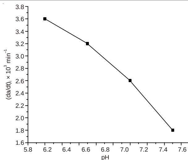
Fig. 2. Effect of pH on the degradation of acid red-14 by HCF(III). Experimental conditions: [acid red-14] = 3.0 \times 10^{-5} mol \text{dm}^{-3} ; [HCF(III)] = 3.0 \times 10^{-6} mol \text{dm}^{-3} ; [Ir nano] = 1.004 \times 10^{-7} mol \text{dm}^{-3} ; Temperature = 40 \pm 0.1 °C
