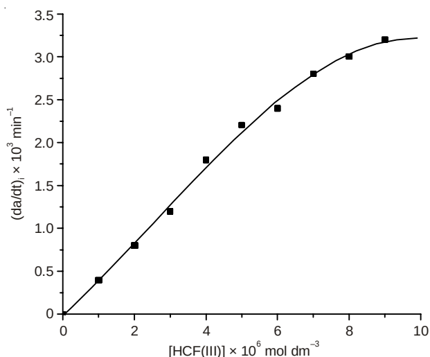
Fig. 3. Effect of [HCF(III)] on the degradation of acid red-14 by HCF(III). Experimental conditions: [acid red-14] = 3.0 \times 10^{-5} mol \text{dm}^{-3} ; [Ir nano] = 1.004 \times 10^{-7} mol \text{dm}^{-3} ; pH = 7.5; Temperature = 40 \pm 0.1 °C
