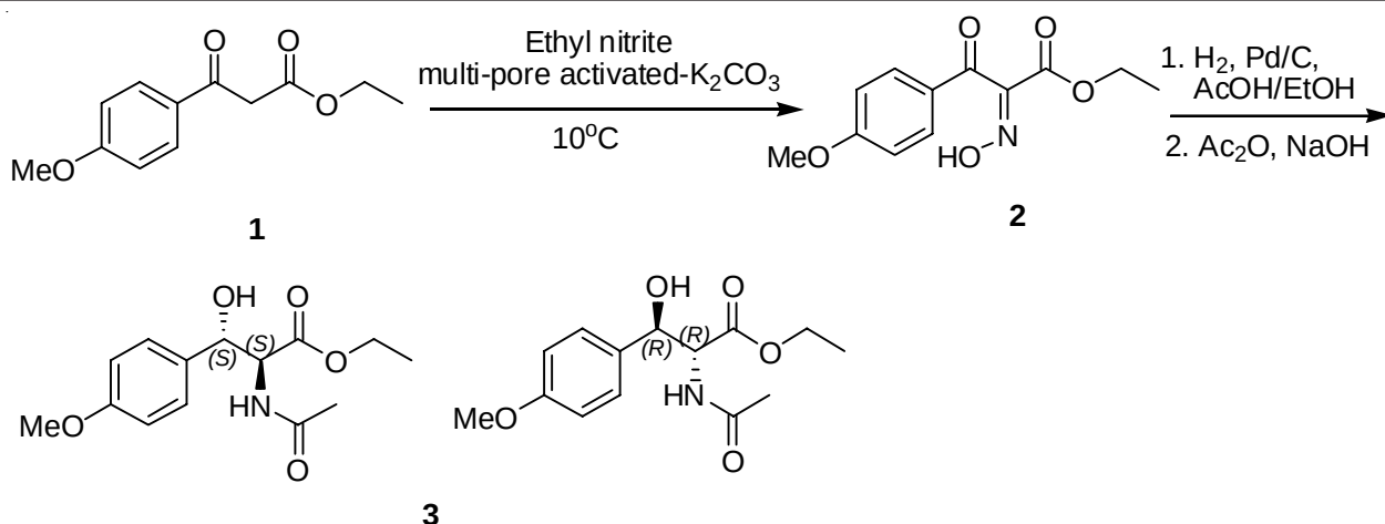
Scheme-I: Synthesis of (±)- erythro - N -acetyl-β-(4-methoxyphenyl)serine ethyl ester 3
