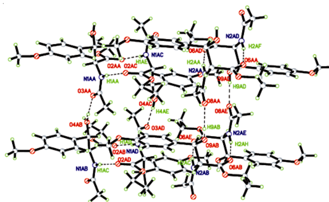
Fig. 4. Hydrogen bonding system between the molecules of 3 . The dashed lines represented the intermolecular hydrogen bonds (H-bonds have been drawn between the donor and acceptor atoms).
