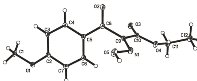
Fig. 1. Molecular structures of oxime 2 , showing the atom-labeling scheme displacement ellipsoids are drawn at the 30 % probability level
