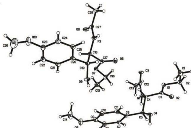
Fig. 3. Molecular structures of compound 3 , showing the atom-labeling scheme. Displacement ellipsoids have been drawn at the 10 % probability level
