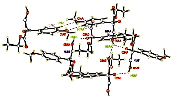
Fig. 2. Hydrogen bonding system between molecules of oxime 2 . The dashed lines represented the intermolecular hydrogen bonds (H-bonds have been drawn between the donor and acceptor atoms)
