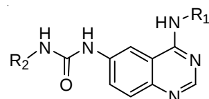
Fig. 1. Structure of compound 6a-j
