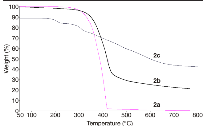
Fig. 2. Thermogravimetric analysis curves of 2a , 2b , 2c at a heating rate 10\text{ }^{\circ}\text{C min}^{-1} in \text{N}_2 atmosphere
