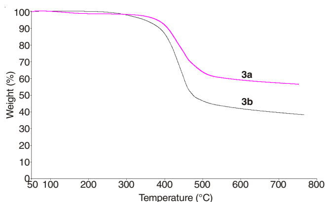
Fig. 3. Thermogravimetric analysis curves of 3a , 3b at a heating rate 10\text{ }^{\circ}\text{C min}^{-1} in \text{N}_2 atmosphere
