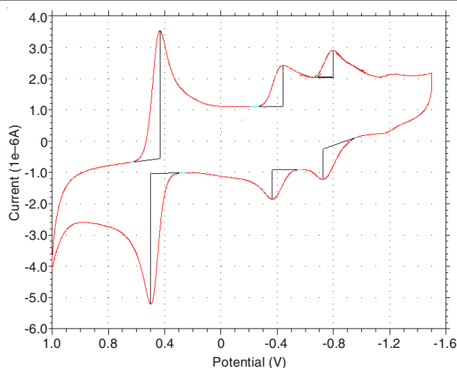
Fig. 1. Cyclic voltammogram of naphthalene-1,4- N -(2-ethylhexyl)-imide- N -ethyl-1 H -benzo[d]imidazol-5-carboxylate ( 3a ) in DMSO, supporting electrolyte 0.2 M sodium perchlorate, scan rate 100 mV s -1 at 25 °C
