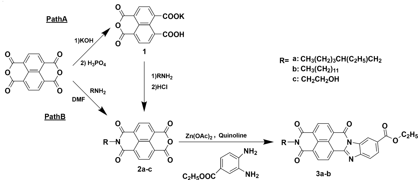
Scheme-I: Synthetic routes of N-alkyl-1,4,5,8-naphthalenetetracarboxylic monoanhydride monoimides ( 2a-c ) and unsymmetrical naphthalene derivatives ( 3a-b )
