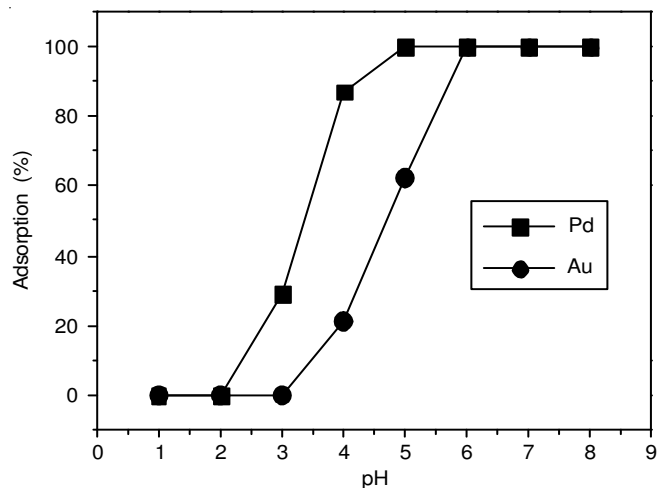
Fig. 1. Effect of pH on the adsorptions
