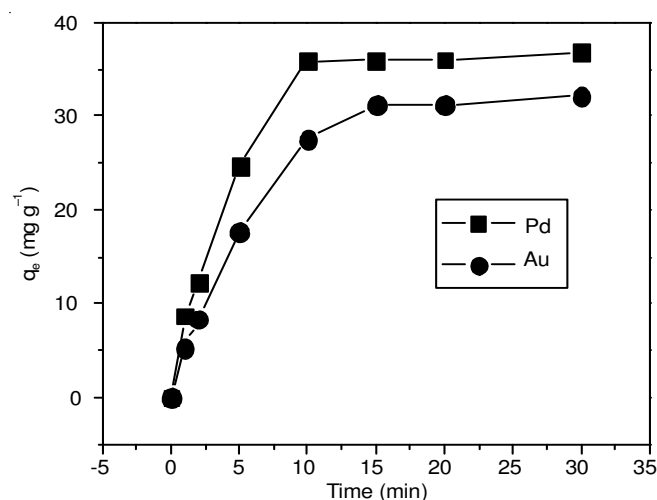
Fig. 2. Effect of contact time on Pd(II) and Au(III) adsorption
