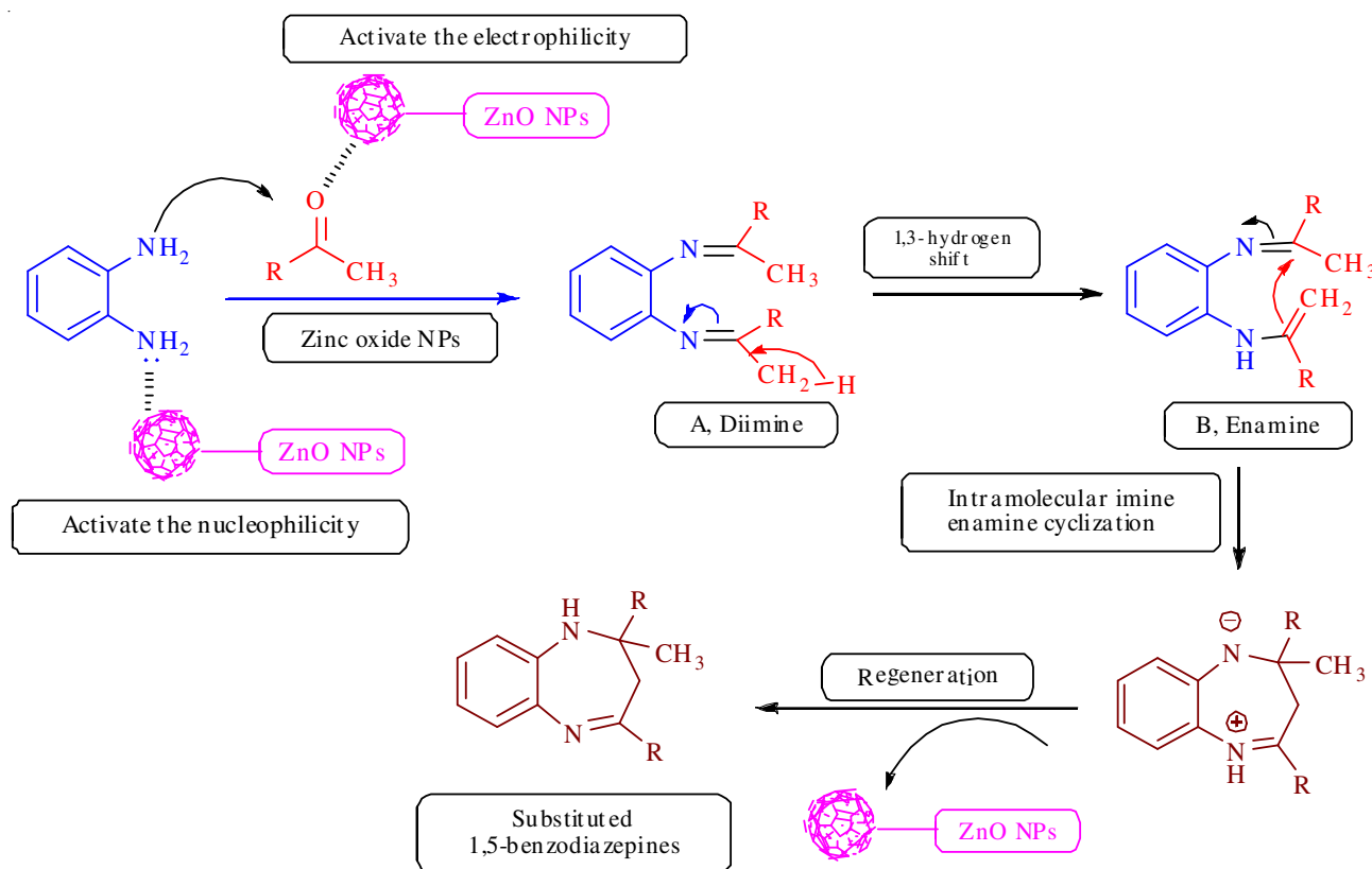
Scheme-II: Proposed mechanism and possible intermediates
