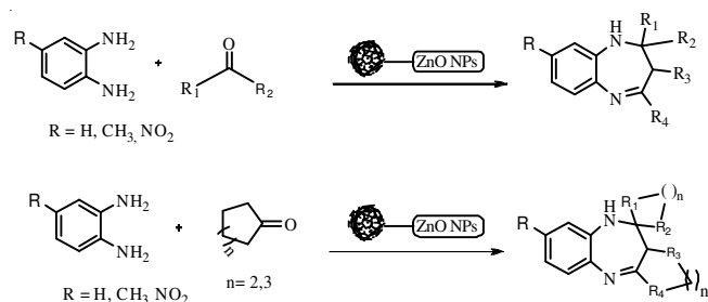
Scheme-I: Chemical reaction for the synthesis of 2,3-dihydro-1H-1,5-benzodiazepines using zinc oxide nanoparticles
