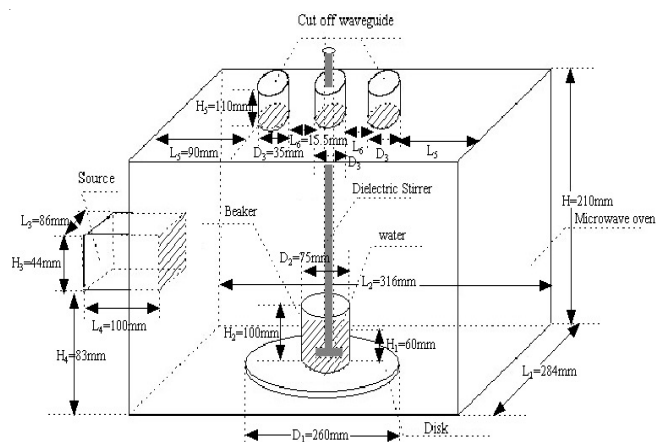
Fig. 2. Schematic of simulation model
