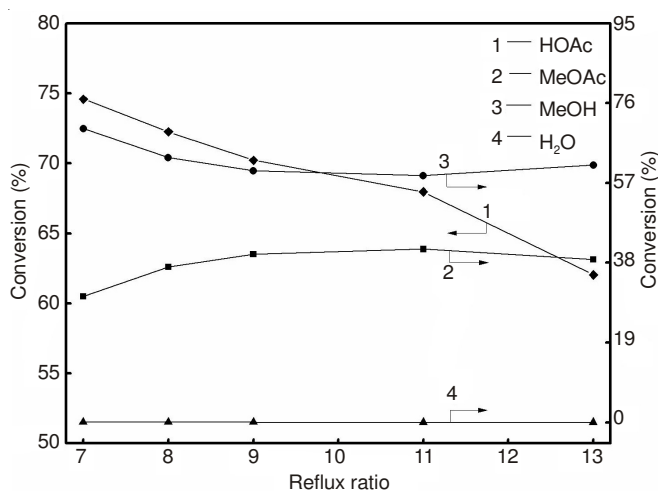
Fig. 6. Effect of reflux ratio on reactive distillation, 1 conversion of HOAc; 2, 3, 4 the distillate composition of MeOAc, MeOH and H 2 O
