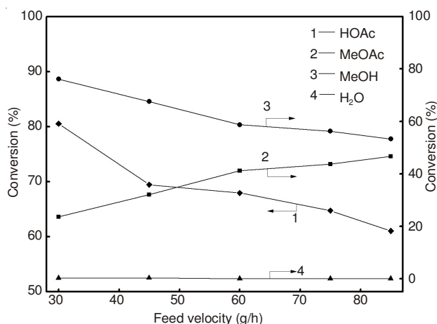
Fig. 3. Effect of diluted acidic acid feed velocity on reactive distillation, 1 conversion of HOAc; 2, 3, 4 the distillate composition of MeOAc, MeOH and H 2 O
