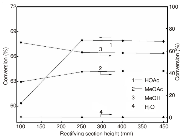
Fig. 5. Effect of rectifying section height on reactive distillation. 1 conversion of HOAc; 2, 3, 4 the distillate composition of MeOAc, MeOH and H 2 O
