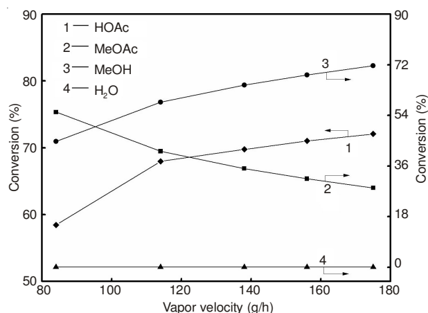
Fig. 4. Effect of MeOH vapor velocity on RD, 1 conversion of HOAc; 2, 3, 4 the distillate composition of MeOAc, MeOH and H 2 O
