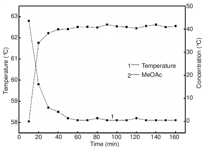
Fig. 7. Equilibrium curves between top temperature, methyl ester content and time
