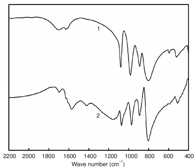
Fig. 2. IR spectrum of PW 12 before (1) and after (2) being loaded on activated carbon
