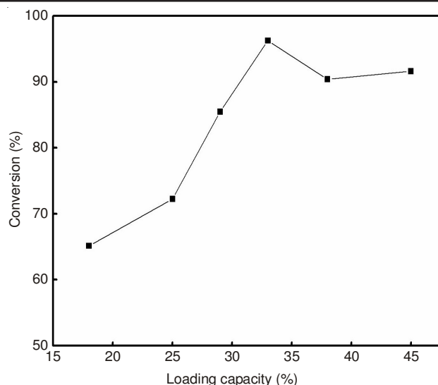
Fig. 1. Influence of PW 12 loadings capacity on the conversion of acidic acid
