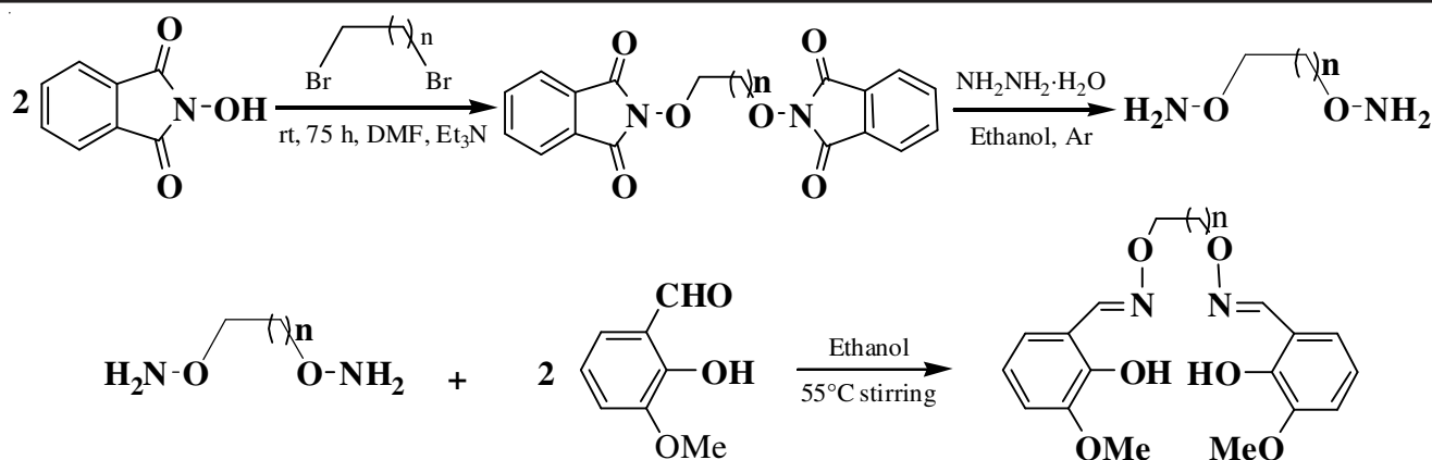
Fig. 1. Synthetic route to Salamo-type bisoxime compounds \text{H}_2\text{L}^1\text{-H}_2\text{L}^4 ( n = 2\text{-}5 )
