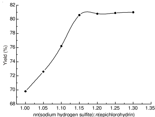
Fig. 2. Effect of the molar ratio on the yield
