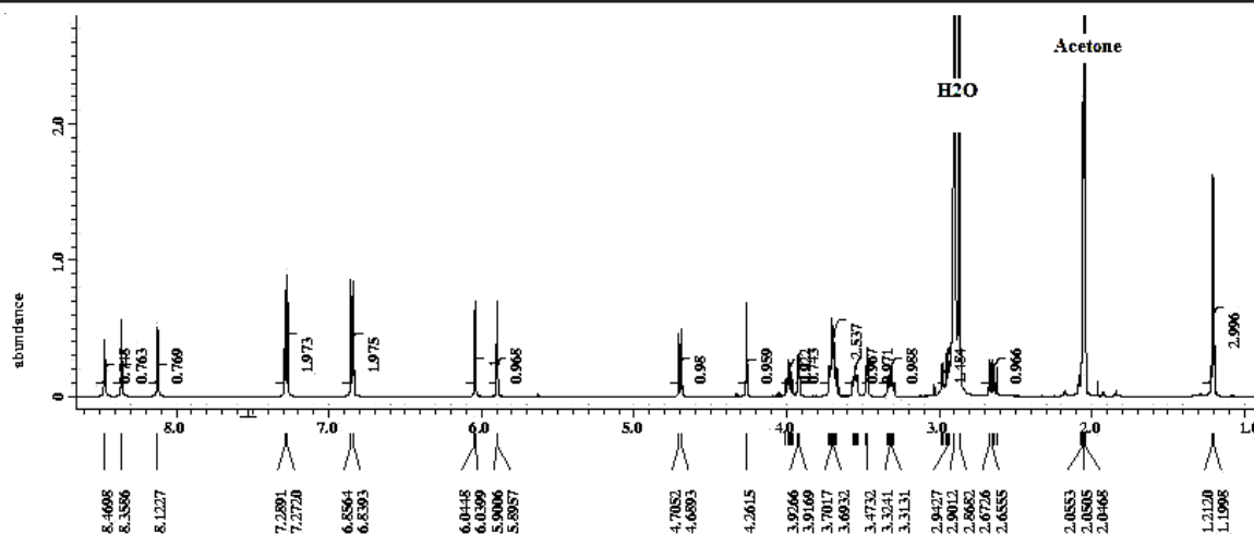
Fig. 3. ^1\text{H} NMR spectrum of compound 1
