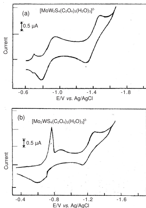
Fig. 4. (a-b) Cyclic voltammogram of [MoW_2S_4(C_2O_4)_3(H_2O)_3]^{2-} and [Mo_2WS_4(C_2O_4)_3(H_2O)_3]^{2-}
