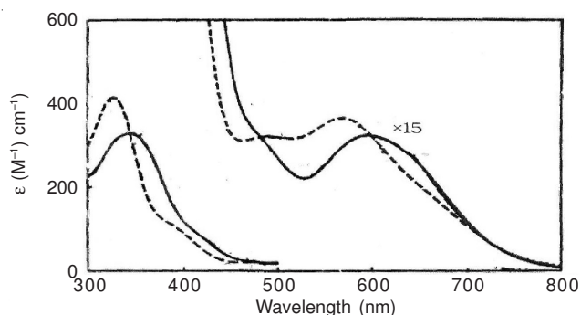
Fig. 2. Electronic spectra of [\text{Mo}_{3-n}\text{W}_n\text{S}_4(\text{H}_2\text{O})_9]^{4+} clusters ( n = 1-2 ) in 2 M HPTS: (—) [\text{Mo}_2\text{WS}_4(\text{H}_2\text{O})_9]^{4+} and (---) [\text{MoW}_2\text{S}_4(\text{H}_2\text{O})_9]^{4+}
