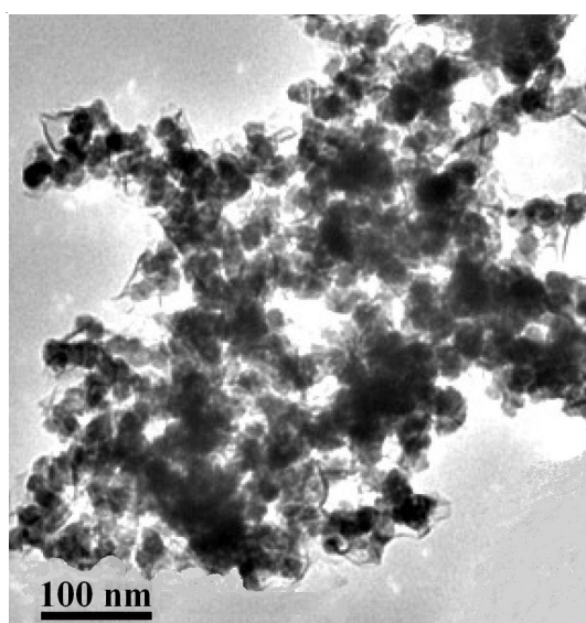
Fig. 3. TEM image of Fe-Ni-Sb-B
