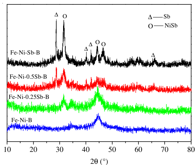
Fig. 1. Powder XRD patterns of Fe-Ni-xSb-B ( x = 1, 0.5, 0.25 and 0) alloy nanoparticles
