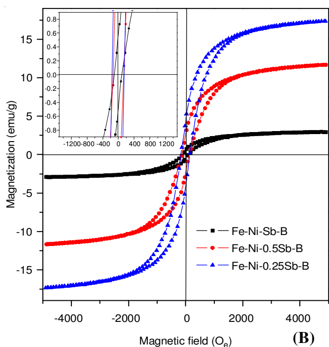
Fig. 4. Magnetic hysteresis curve of the Fe-Ni-Sb-B nanoalloy (A) and the hysteresis loops of the alloys with different mole ratio of the metal salts (B)
