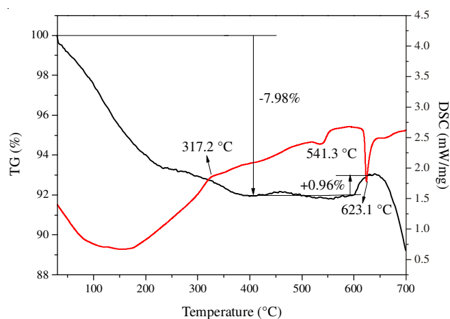
Fig. 2. TG-DSC curves of Fe-Ni-Sb-B
