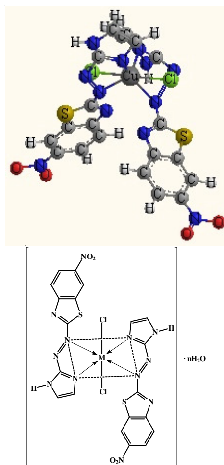
Fig. 12. The proposed chemical formula of chelet complexes when:- M = Co(II), Cu(II), Cd(II) and Hg(II); n = 1; M = Ni(II) and Zn(II); n = 0
