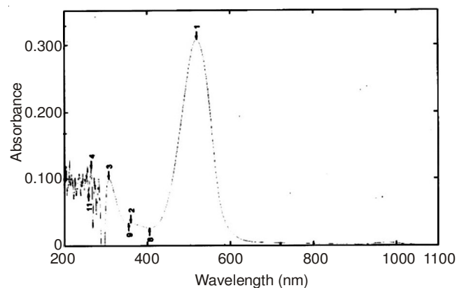
Fig. 11. UV-visible spectrum of Cd(II)-Complex
