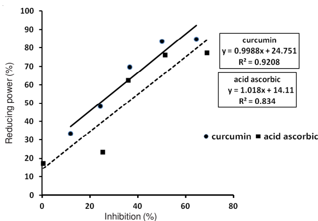
Fig. 4. Correlation between DPPH and reducing power activity for curcumin and ascorbic acid by regression analysis
