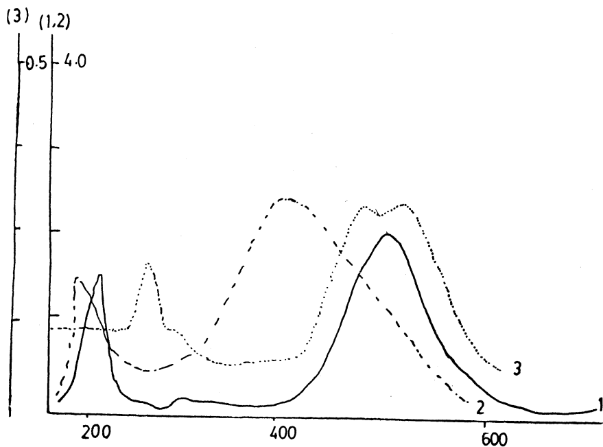
Fig. 1. Absorption spectra
