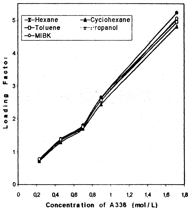
Fig. 3. Variation of loading factors with concentration of Alamine 336 in different diluting solvents.
