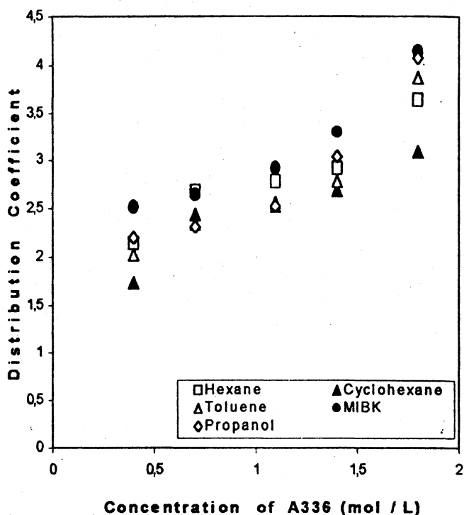
Fig. 2. Variation of distribution coefficients with concentration of Alamine 336 in different diluting solvents.
