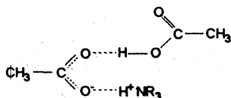
Fig. 1. The structure of acid : amine complex
