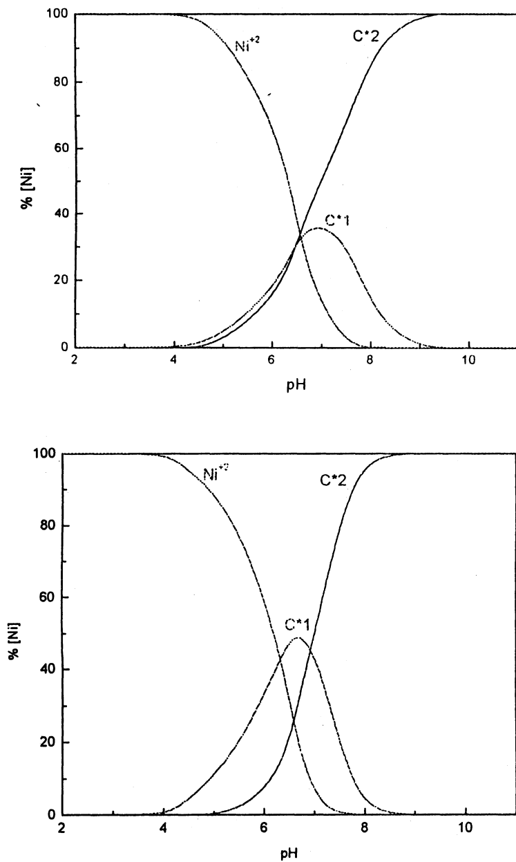
Fig. 3. Species distribution diagrams as function of pH for ternary complexes:
