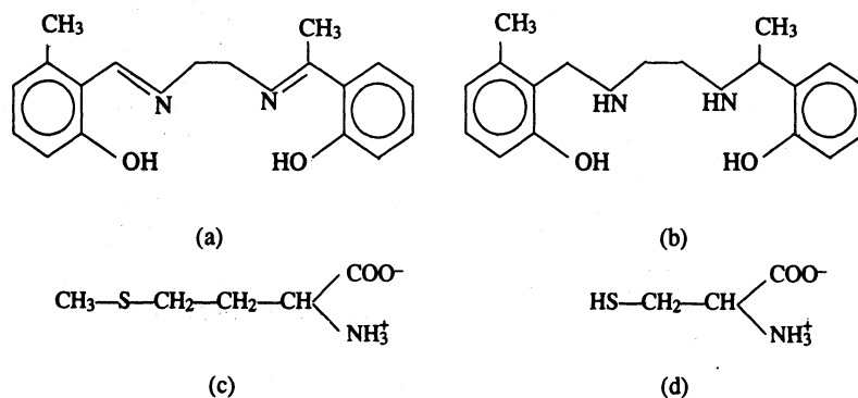
Fig. 1. Structure of ligands: (a) H_2BS : N,N' -bis(2-hydroxy acetophenon)ethylenediimine, (b) H_2BSR : N,N' -bis(2-hydroxy acetophenyl)-1,2-diaminoethane, (c) Met: Methionine, (d) Cys: Cysteine
