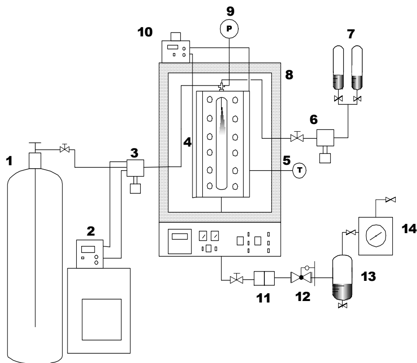
Fig. 2. Schematic diagram of the ASES apparatus
