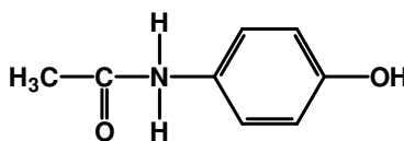
Fig. 1. Chemical structure of acetaminophen
