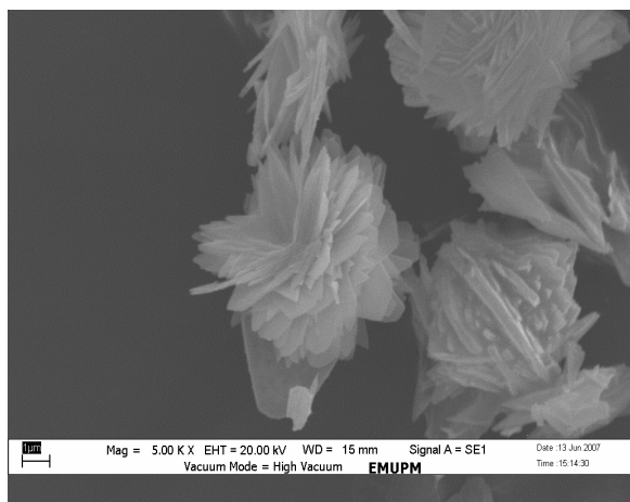
Fig. 5: SEM micrograph of VPD (with 5000 \times magnification)
