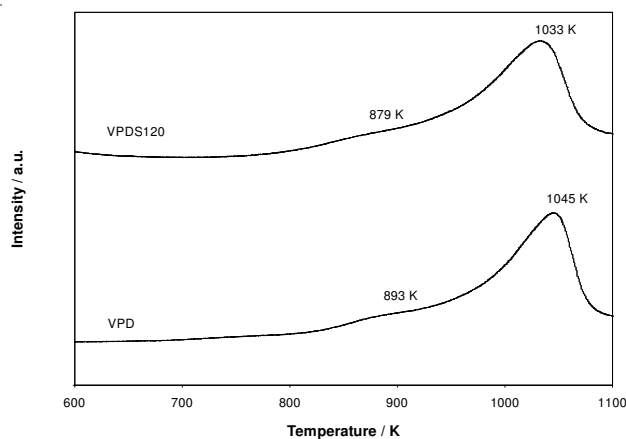
Fig. 8. TPR profiles for VPD and VPDS120 catalysts
