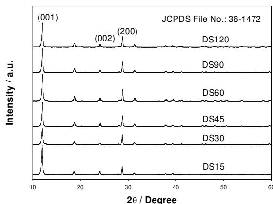
Fig. 1: XRD patterns of sonochemical synthesized vanadyl phosphate dihydrate (DS15-DS120)
