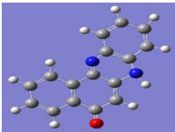
Fig. 1. 10,12-Dihydro-5-10-diazatetraphene-12-one (DHD)
